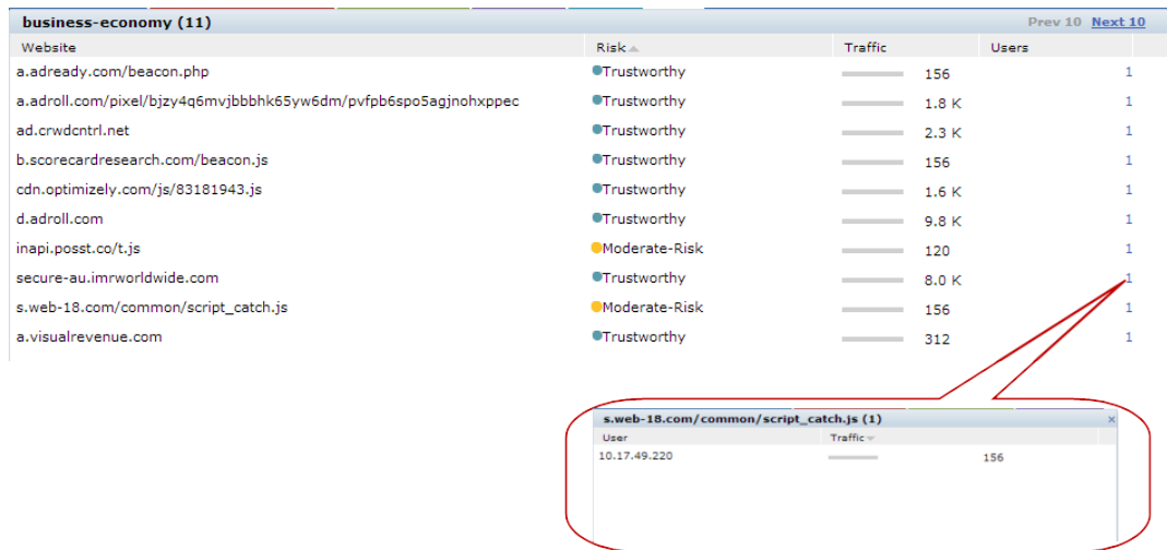
Figure 162 User Table
