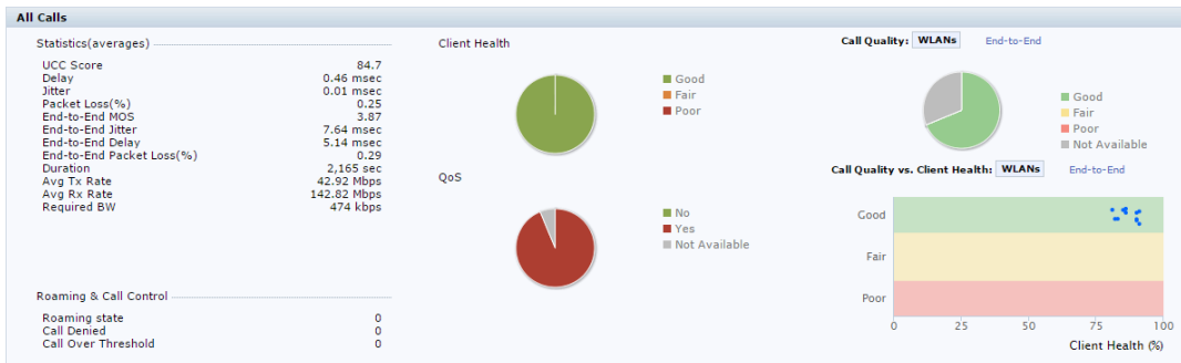
Figure 206 All Calls
