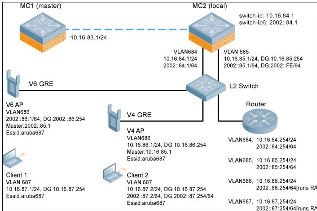
Figure 34 IPv6 Topology
